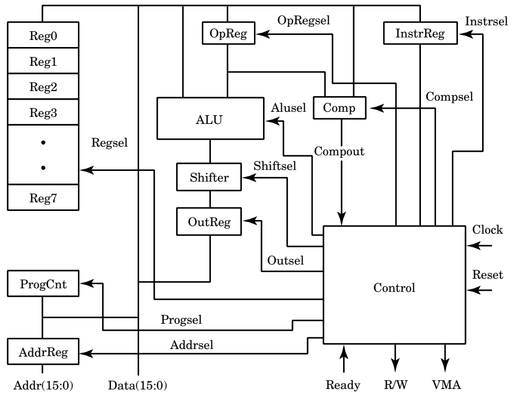
Figure 13-1 CPU Block Diagram.
