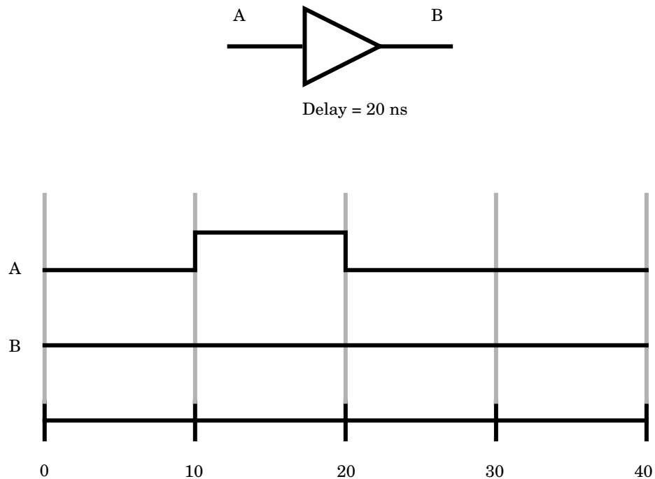
Figure 2-4 Inertial Delay Buffer Waveforms.
