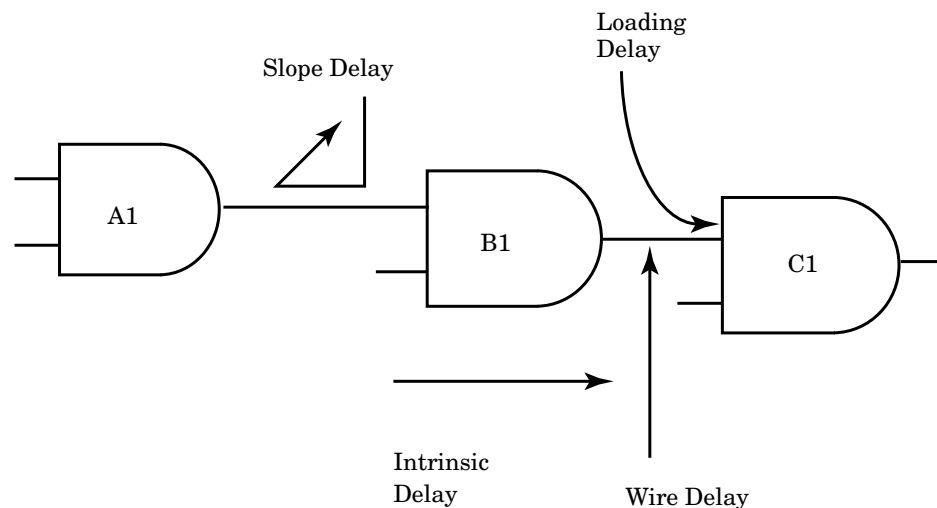
Figure 9-7 Delay Effects Used in Delay Model.
