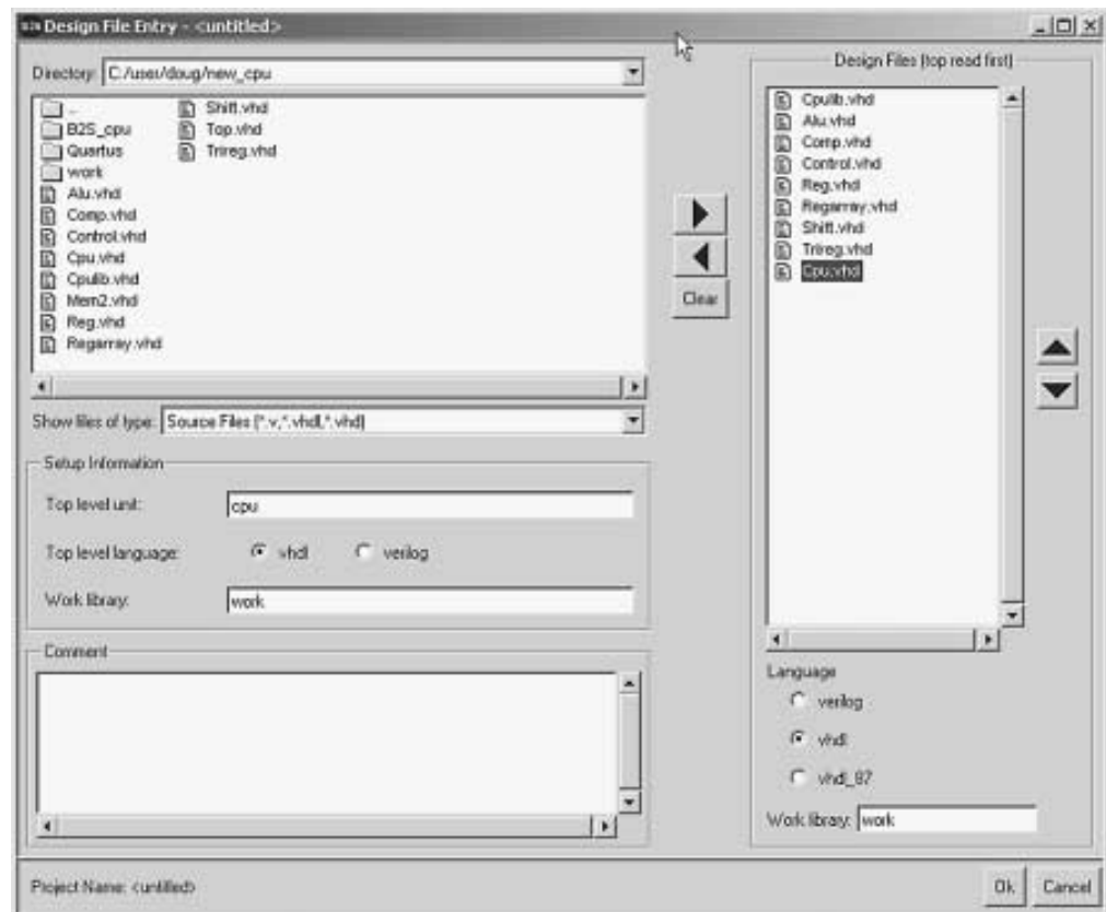
Figure 18-5 Top Level Unit and Language Specified.
