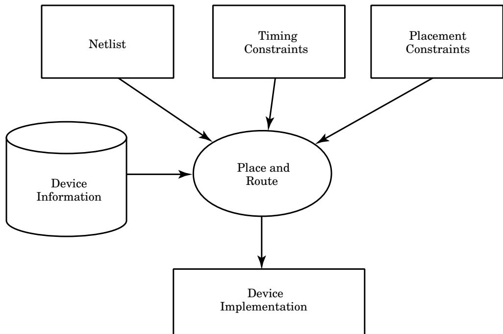
Figure 11-5 Place and Route Data Flow.
