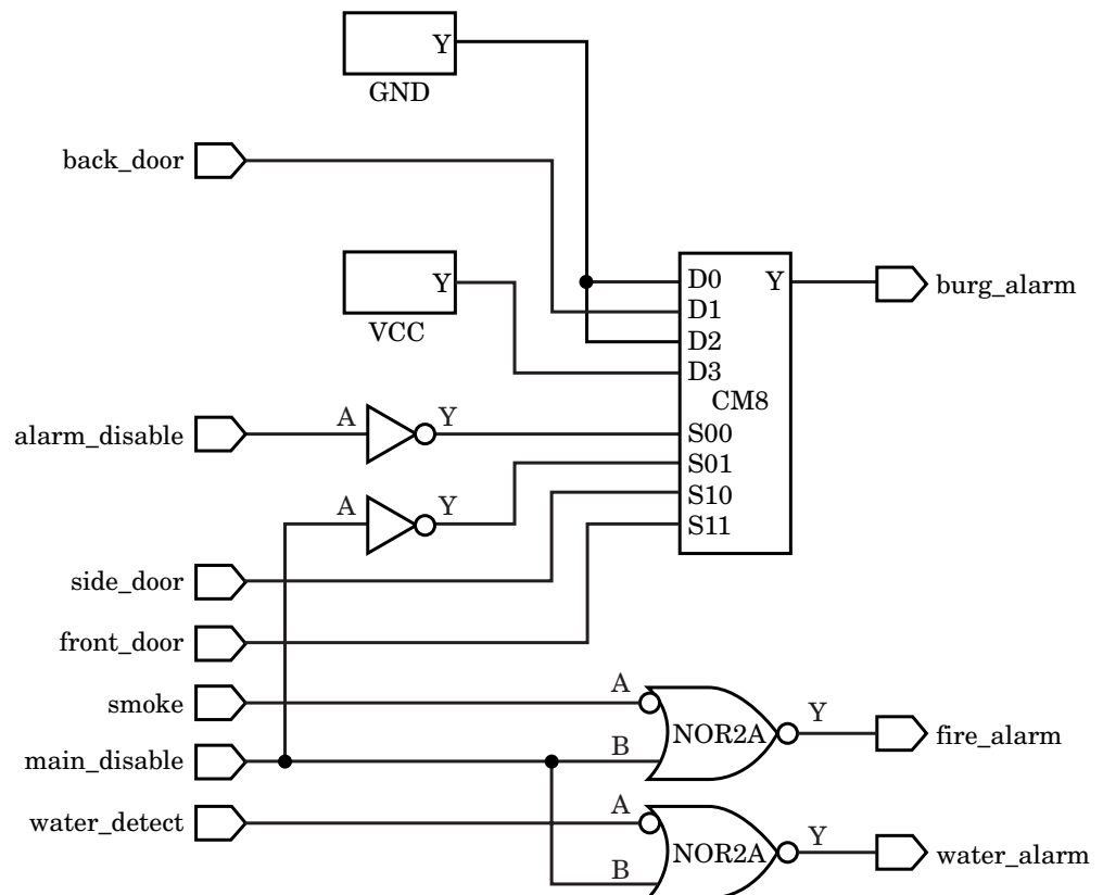
Figure 10-4 A sample synthesized output.
