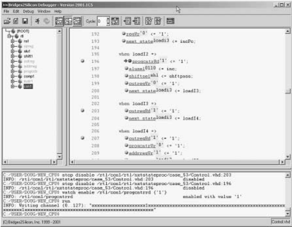
Figure 18-13 Trigger on progcntrRd Watchpoint.
