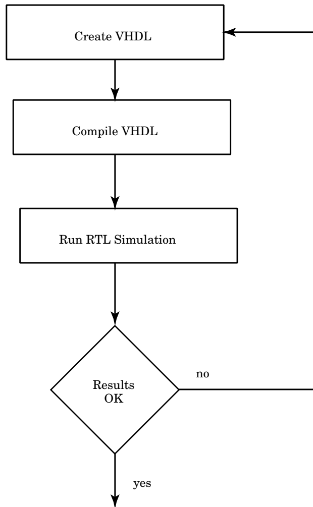
Figure 11-2 RTL Simulation Flow.
