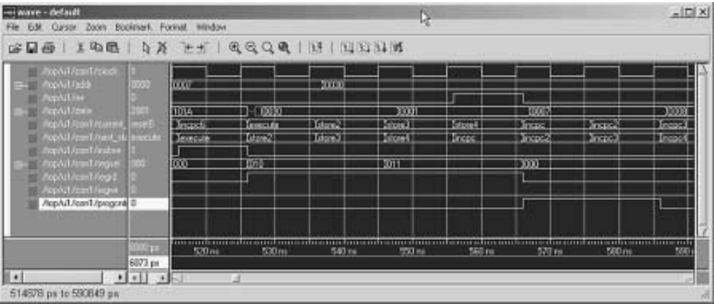
Figure 14-7 A Waveform Display Showing the Store Instruction.
