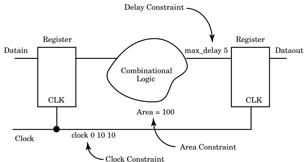
Figure 9-5 Register and Cloud Diagram with Con- straints.
