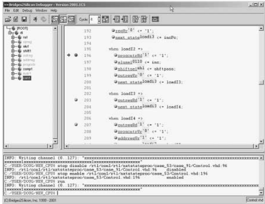
Figure 18-10 Trigger on LoadI2 and Captured Data Displayed.
