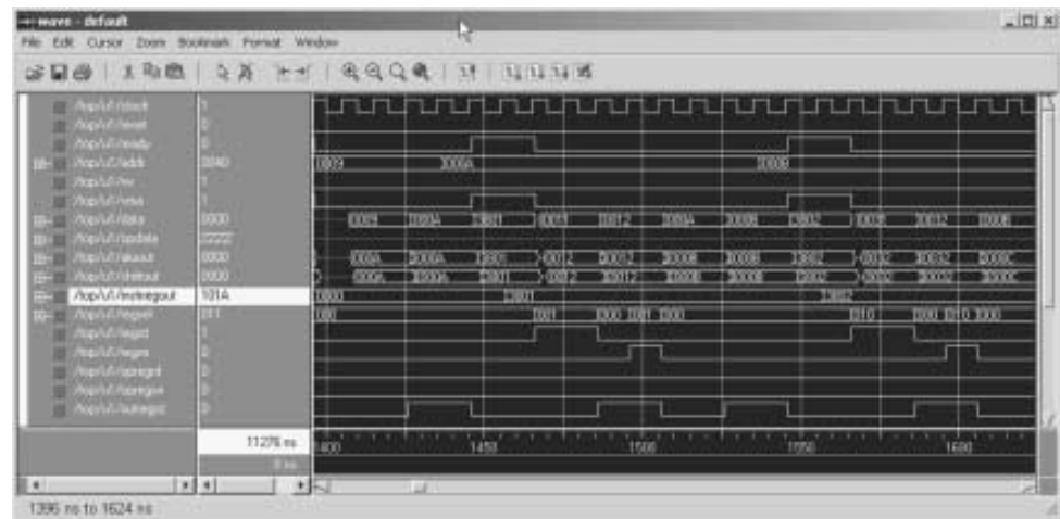
Figure 11-3 Sample Waveform Output.
