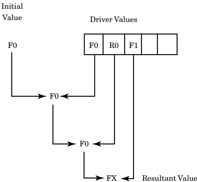
Figure 5-5 Nine State Resolution with Three Values.
