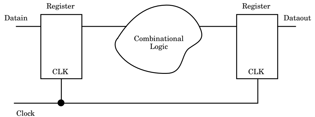
Figure 9-2 Register and Cloud Diagram.
