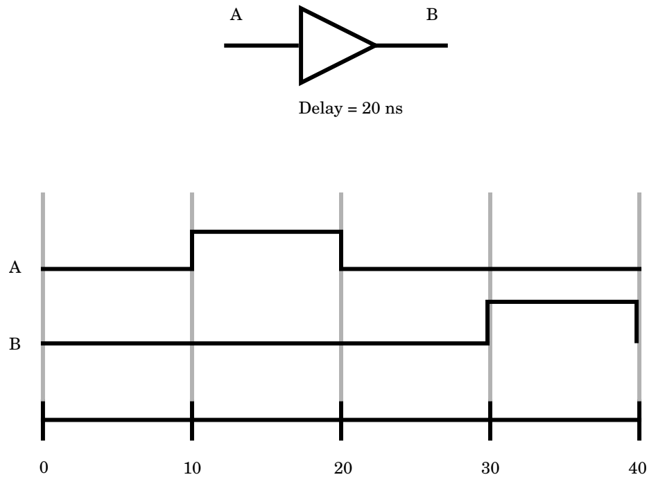
Figure 2-5 Transport Delay Buffer Waveforms.
