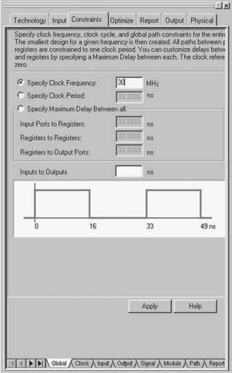
Figure 15-7 Set Clock Constraint to 30 Mhz.
