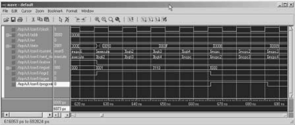
Figure 14-8 Branch Instruction execution.
