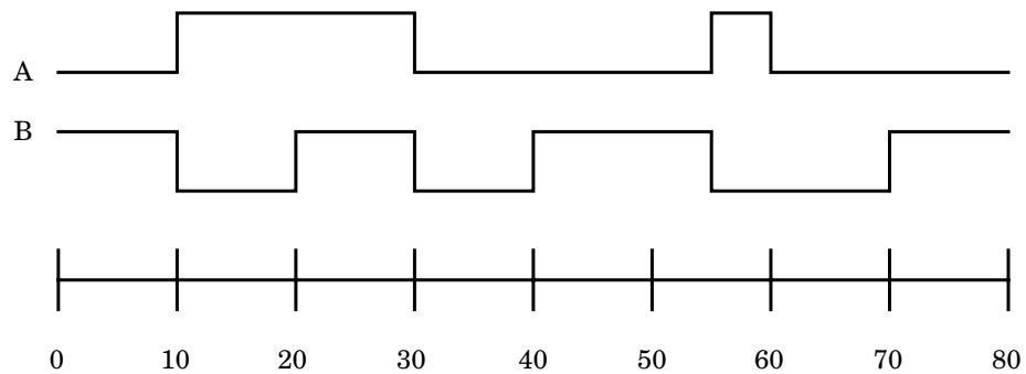
Figure 6-3 Example Showing 'DELAYED' (10ns).
