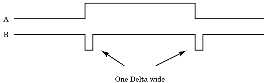
Figure 6-4 Example Showing 'DELAYED' (0 ns).
