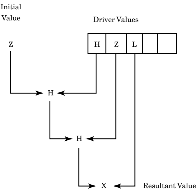
Figure 5-3 Four State Resolution with Three Values.
