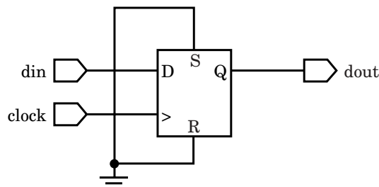
Figure 10-6 The Output of the Leonardo Synthesis Tool.
