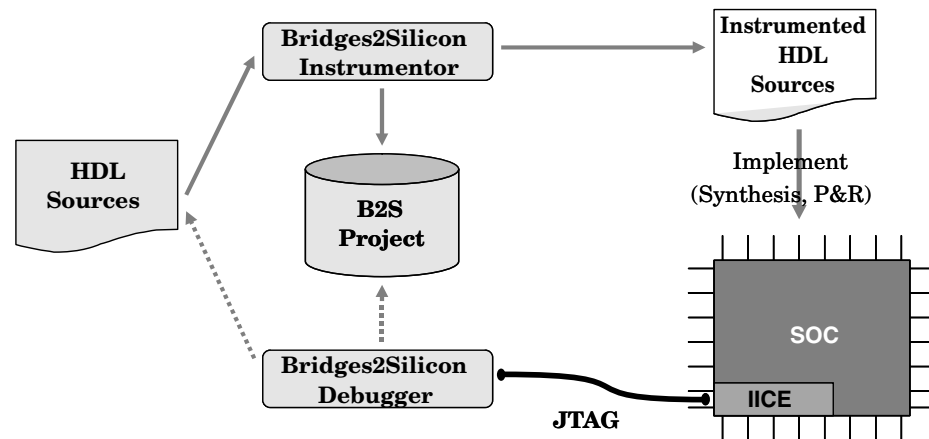
Figure 18-2 Bridges2Silicon Debugger Overview.
