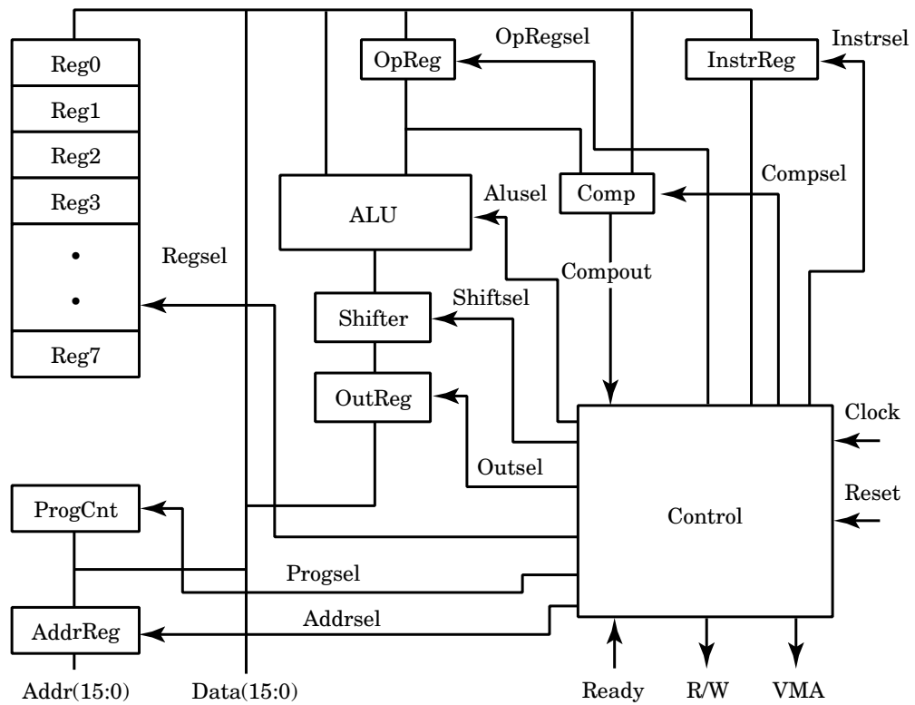
Figure 12-1 CPU Block Diagram.
