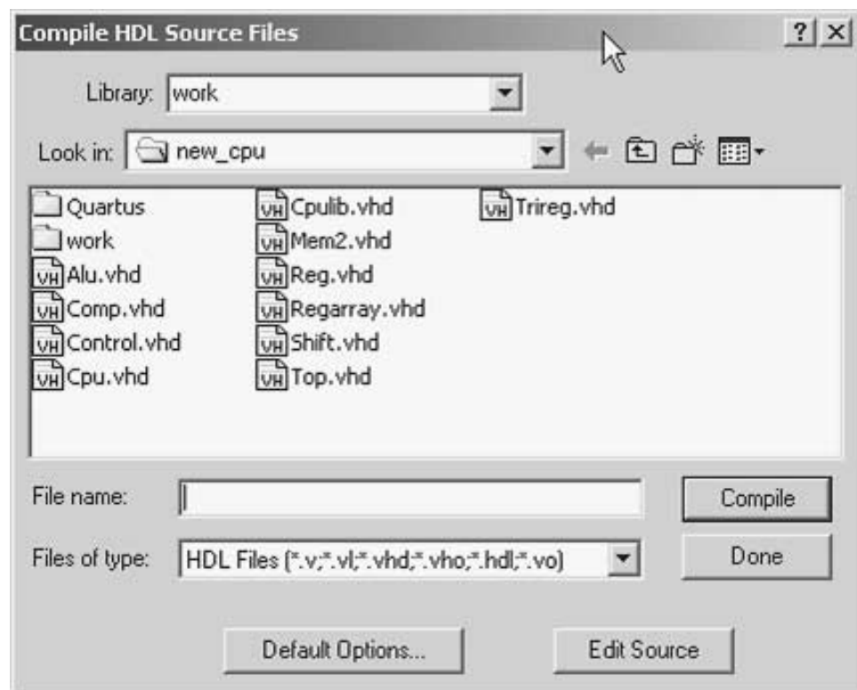
Figure 14-4 Compile VHDL Source Dialog Box.
